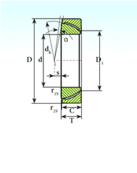
GAC 220 CP Bearing 2D drawings and 3D CAD models
