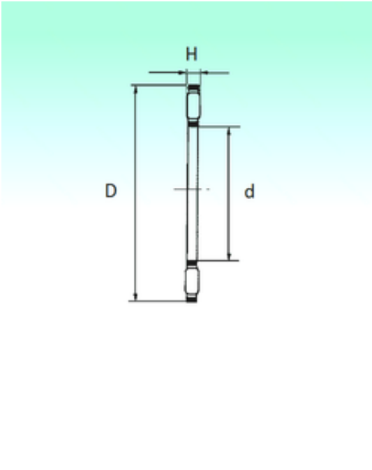
AXK 1024 Bearing 2D drawings and 3D CAD models
